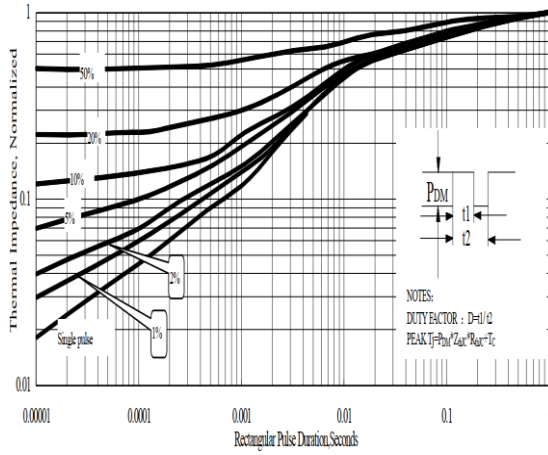
Fig 15 Maximum transient thermal impedance (TO-220AB / TO-263)
