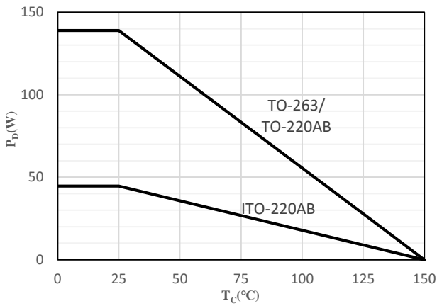
Fig 1 Power Dissipation
