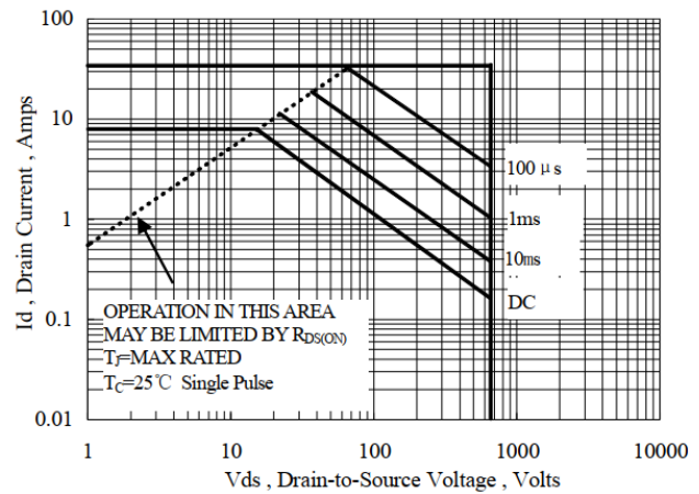
Fig 14 Safe Operating Area (ITO-220AB)
