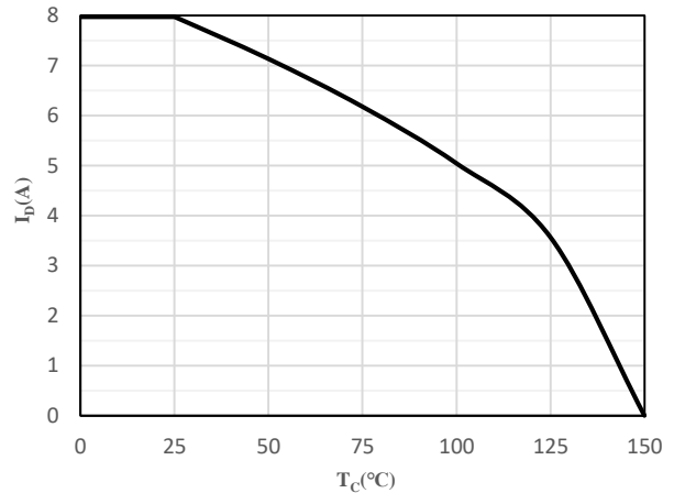
Fig 2 Drain Current
