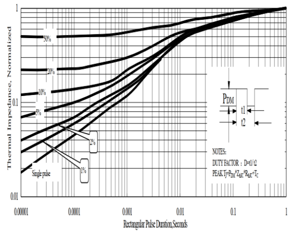
Fig 16 Maximum transient thermal impedance (ITO-220AB)
