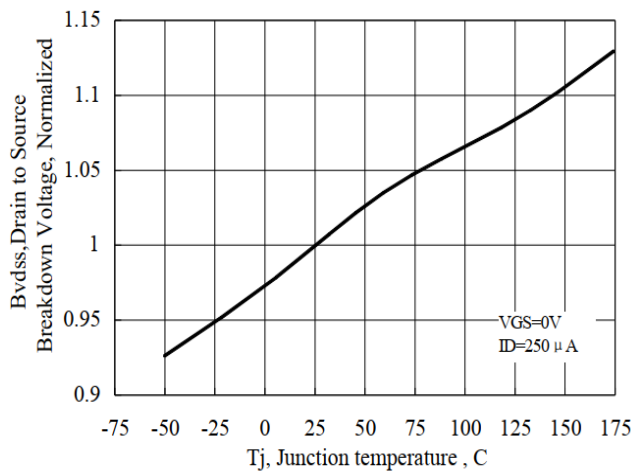
Fig 11 Normalized Breakdown Voltage vs. Junction Temperature
