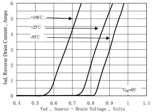
Fig 6 Body-Diode Characteristics
